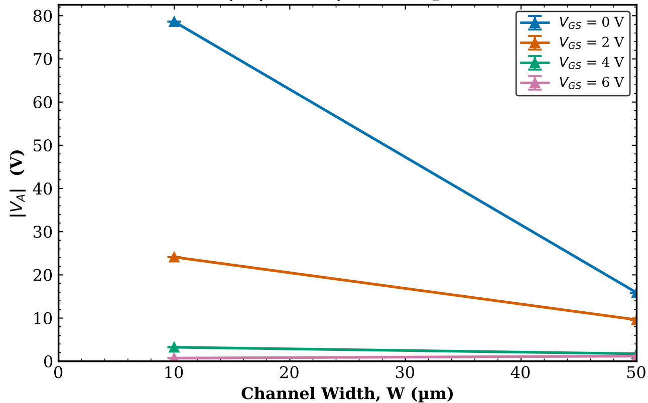
TFT2 Transistor 1 |V_A| vs W | L = 20\text{ }\mu\text{m}
